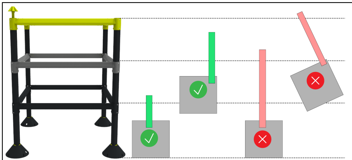
Figure SG3-1: Examples of legal and illegal vertical expansion.
