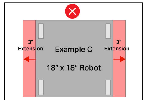
Fig SG2-3: This is not legal. Expanding out two sides is not permitted, even if the Robot maintains 18" x 24" overall dimensions.
